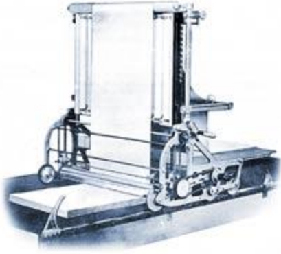
Utica Tubular Spreading Machine
